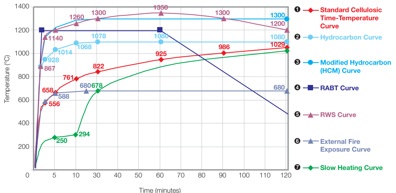
Fire Curves
